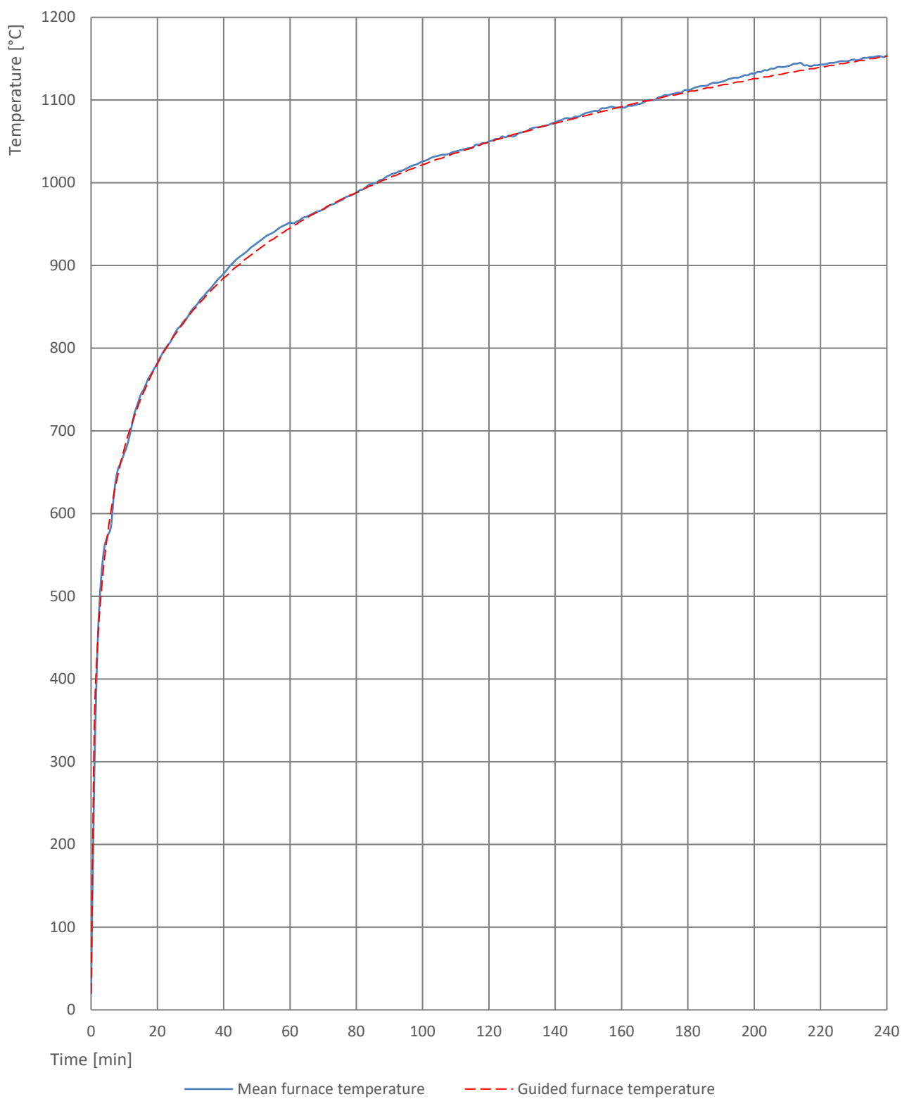
Figure 1. Furnace temperature.
