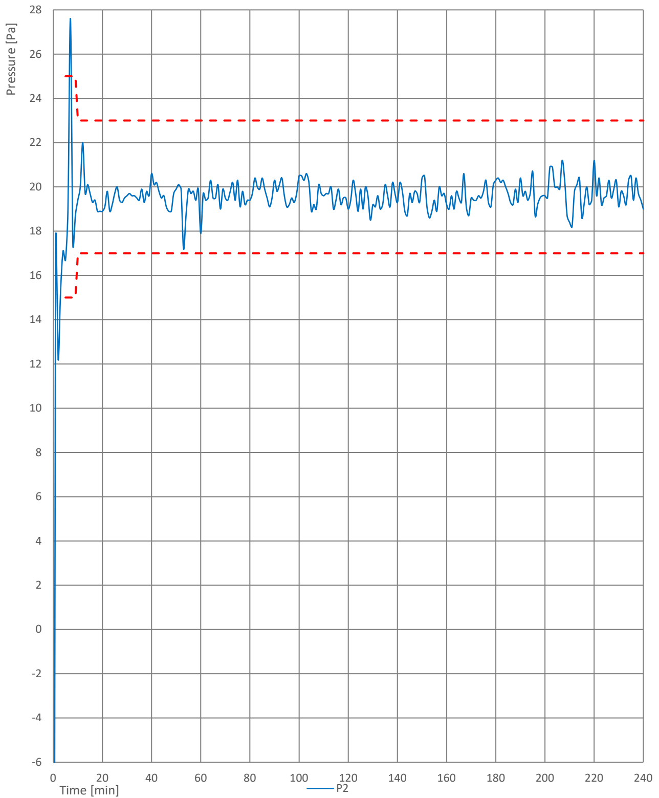
Figure 1. Pressure difference.
