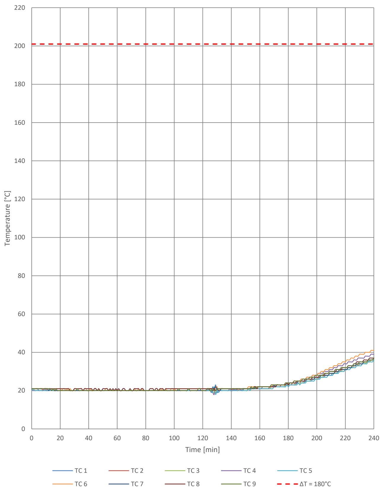
Figure 2. Measured specimen surface temperatures, TC1...TC9.
